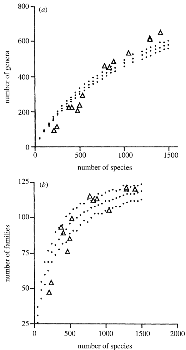
Figure 4. Relation of species richness to generic richness ( a ) and familial richness ( b ) for eastern Pacific benthic molluscs. The dotted lines represent the mean expectation with 95% confidence interval produced by a random resampling (with replacement) of our entire data set. The resampling was done in increments of 50 species; 100 iterations were run for each sampling level. The triangles represent observed values. For both genera and families, high-diversity assemblages tend to have more higher taxa than expected whereas low-diversity ones have fewer higher taxa than expected (see also text).
