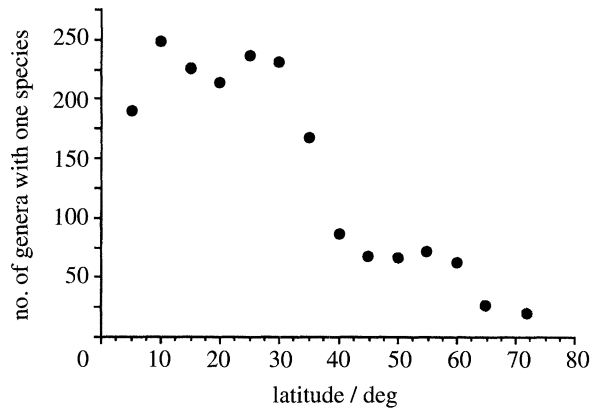
Figure 7. Latitudinal distribution of genera with only one eastern Pacific species. Each points represents the number of such genera present in a 5 deg latitudinal band.
